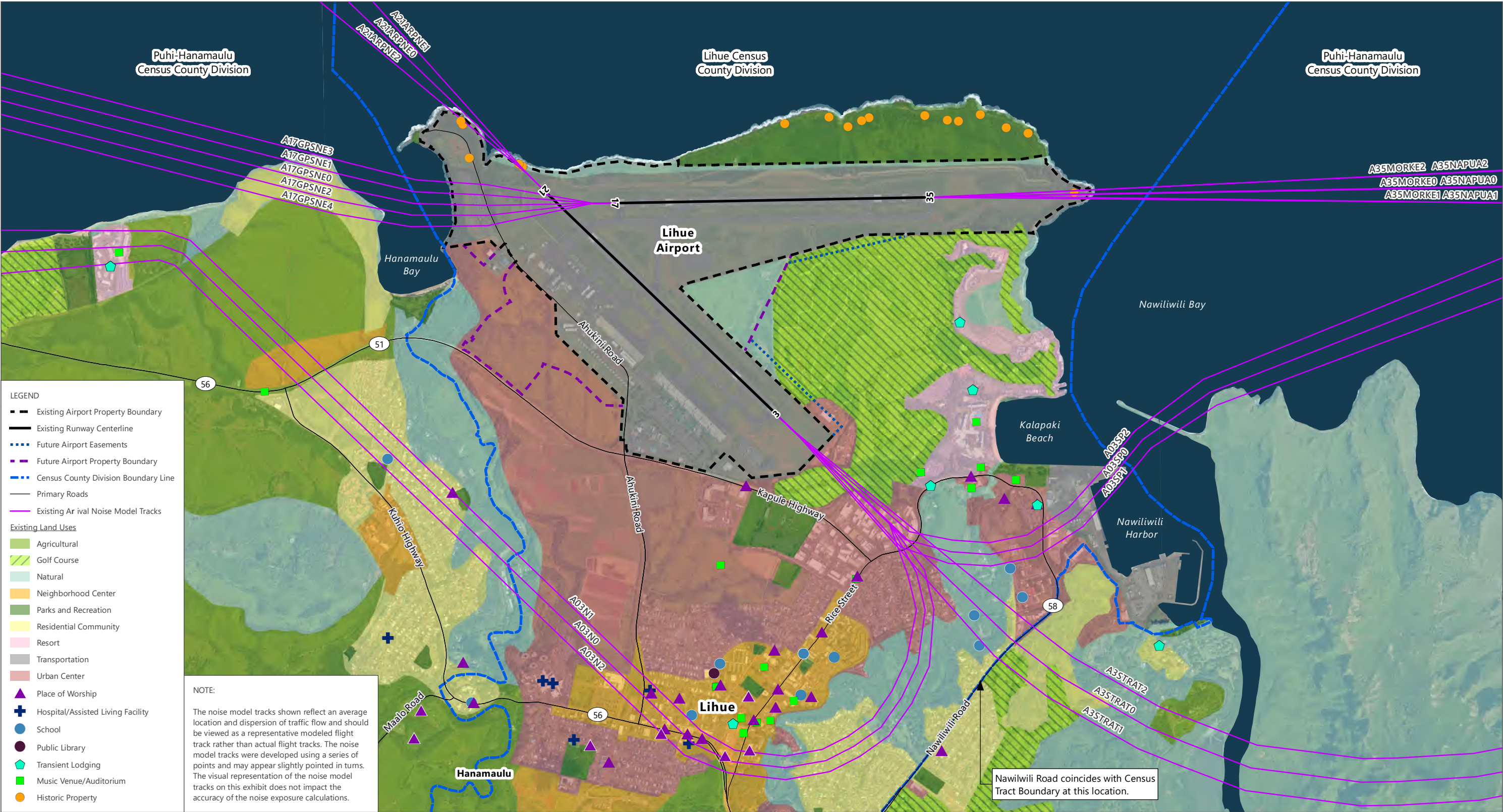
EXHIBIT 2.7-2 GENERALIZED FIXED-WING AIRCRAFT ARRIVAL NOISE MODEL TRACKS – 2019 EXISTING CONDITION
